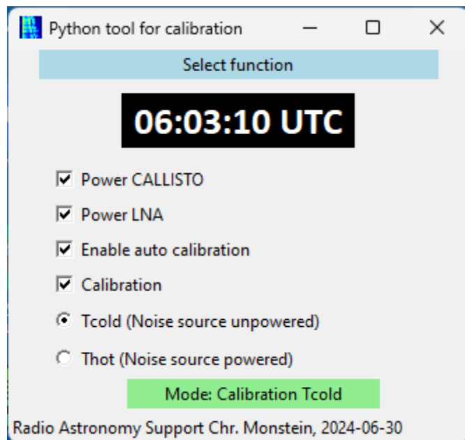
Fig. 8: Python application MOS-ctrl.pyw to control calibration unit, Callisto and LNA2000. There is also a C++ version available but, it doesn't work properly on Windows 11, only Win XP, 7, 8 and 10.
