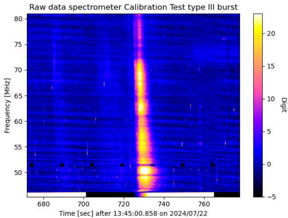
Fig. 11: Zoom into raw data (FIT-file from CALLISTO) before calibration. Intensity in digits.
