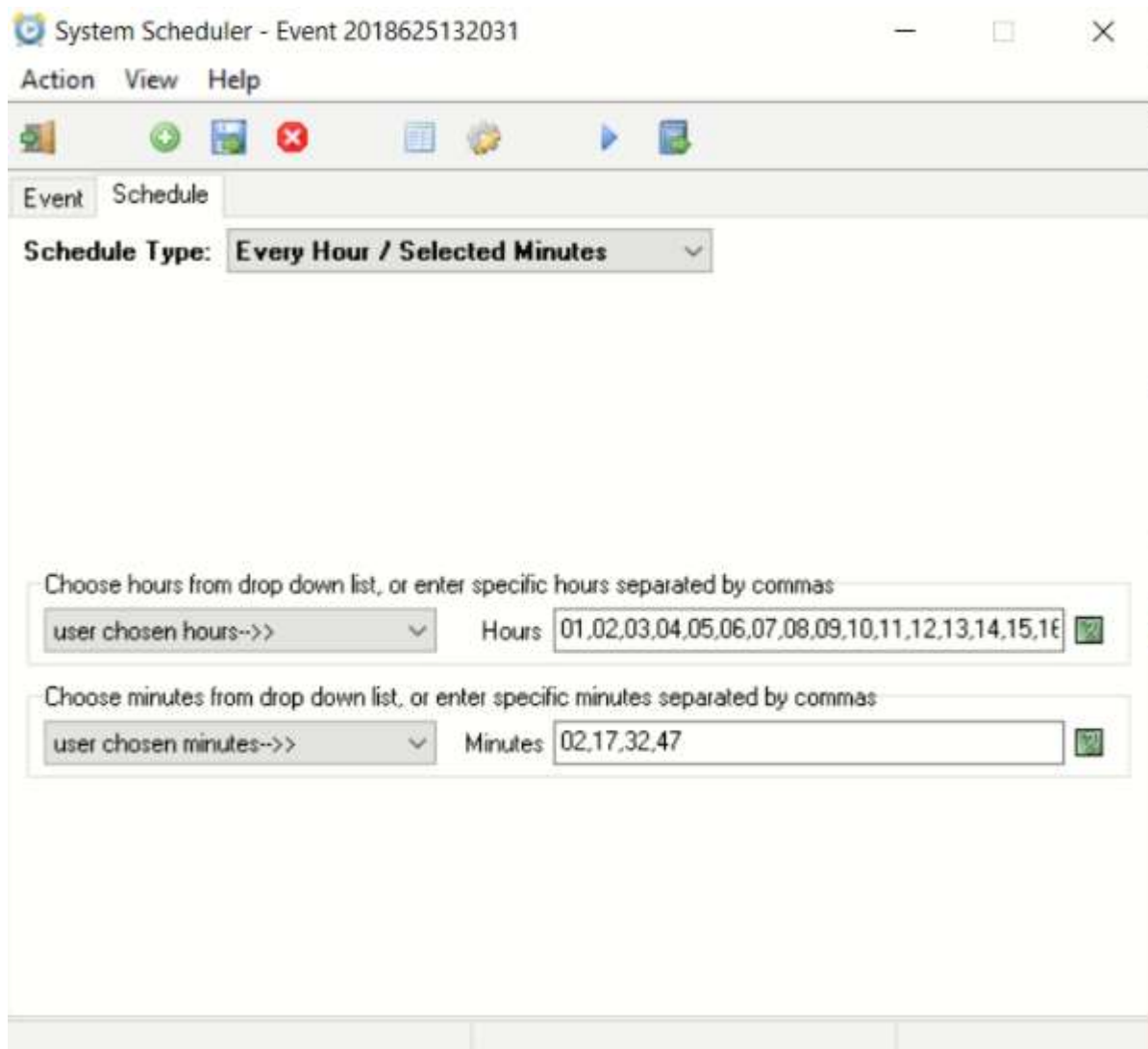
Fig. 21: Scheduling for FTP-upload
