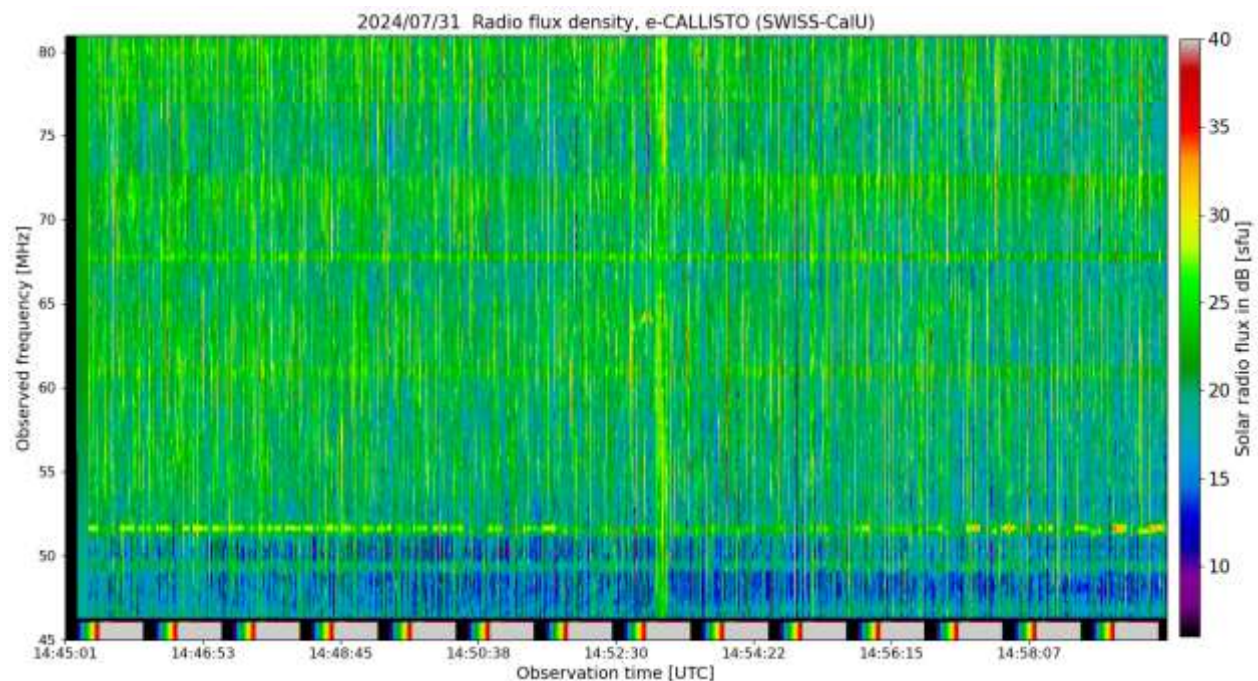
Fig. 17: Heavy lightning in the afternoon at a distance of 1...2 km. On the far-left side we can see 10 seconds Tcold with ~300 kelvin (black), followed by Thot ~12'000 kelvin for another 10 seconds (green). Antenna temperature of lightning strikes exceeds 12'000 kelvins.
