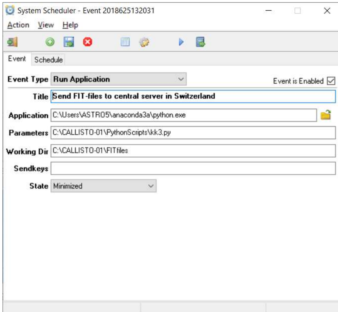
Fig. 20: Application configuration for FIT-file upload to central server. Path to Python.exe might be different for every user. You need to search for python.exe using file-explorer. Parameter-folder as well as working folder might also look different, depending on chosen drive and instrument-code = focus-code (00...63).
