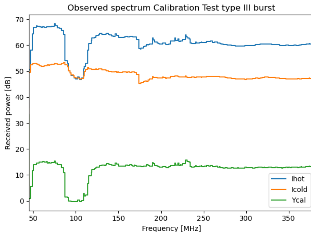
Fig. 9: Calibration signals with notch-filter at FM 88 – 108 MHz and low pass filter at 450 MHz to avoid saturation of LNA and/or CALLISTO by commercial transmission services. Ycal denotes to received Y-factor Thot/Tcold = Ihot/Icold
