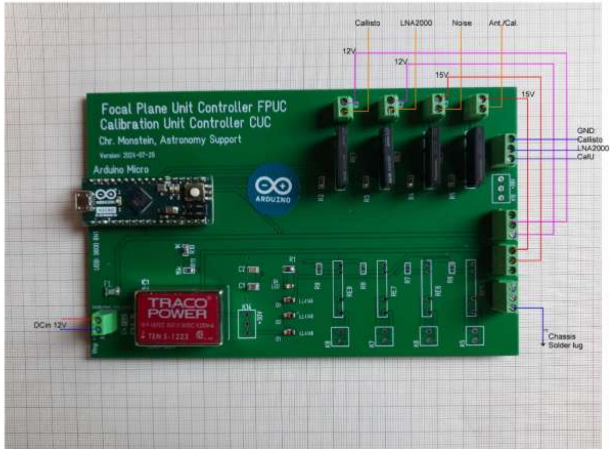
Fig. 22: Harnessing of CuC inside aluminium enclosure. Be aware that all supply voltages (purple and red wires) have to be connected the outer contacts of K1.... K4 due to internal diode of the MOS-relay. Inner contacts (orange wires) need to be connected with the connectors at the back-plate of the enclosure! Blue wires denote to ground connections.
