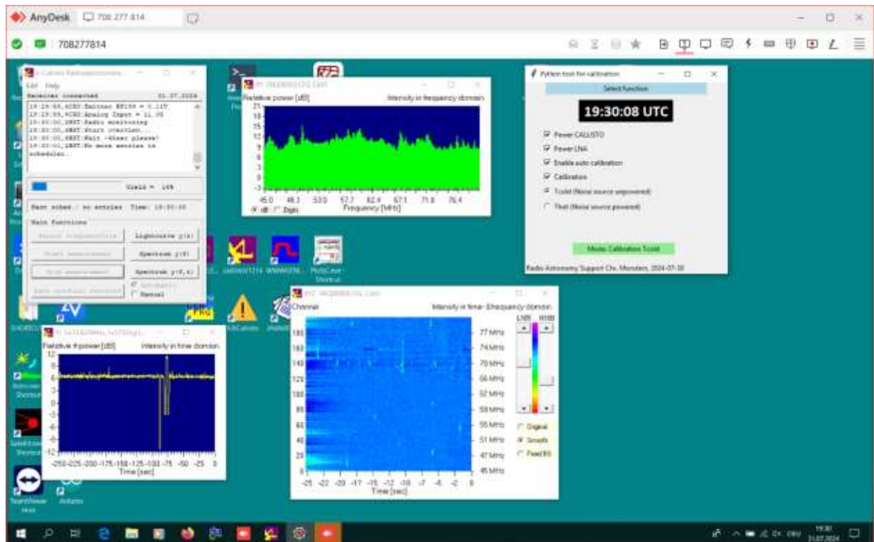
Fig. 10: Running CALLISTO application (C++) and control application (top right in Python3). Image = remote screen-shot via AnyDesk. Light curve bottom left shows a calibration sequence Tcold, Thot.
