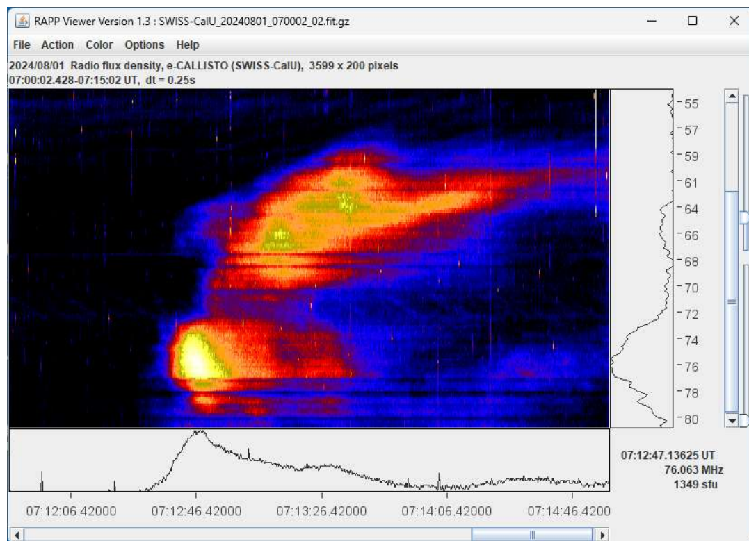
Fig. 16: Calibrated type II radio burst during Swiss National Holiday. Peak flux 1349 sfu at 76 MHz at position of mouse cursor at 07:12:47 UT. Plot presented as screen-hot from JavaViewer https://e-callisto.org/Software/jv_20070109.jar
