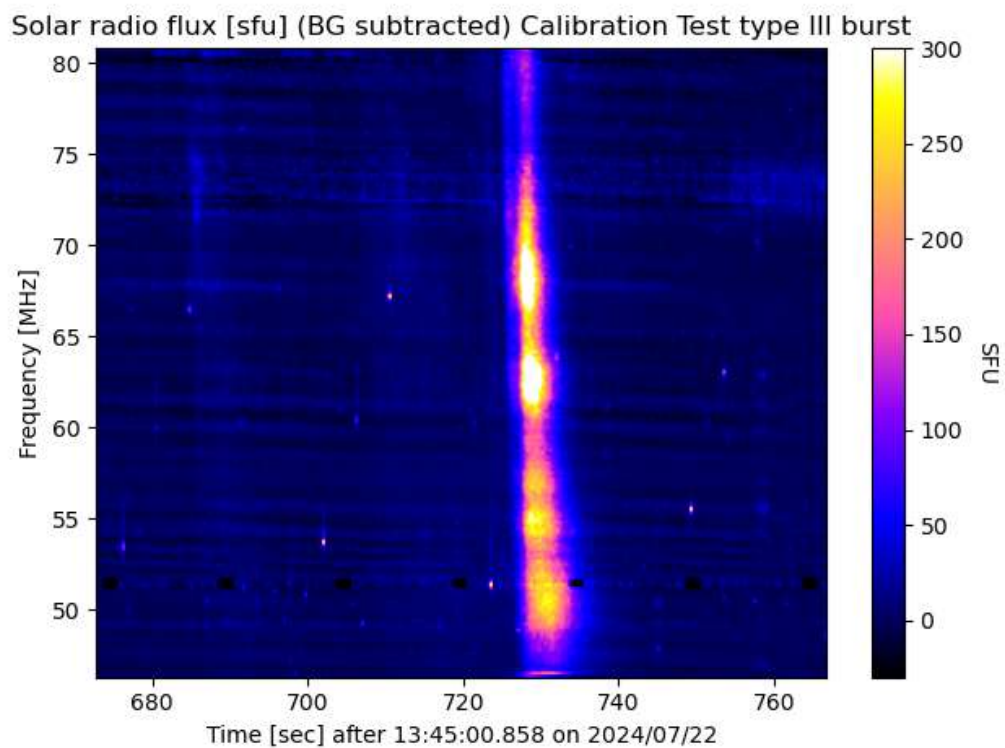
Fig. 14: Calibration in SFU, plot: with background subtracted
