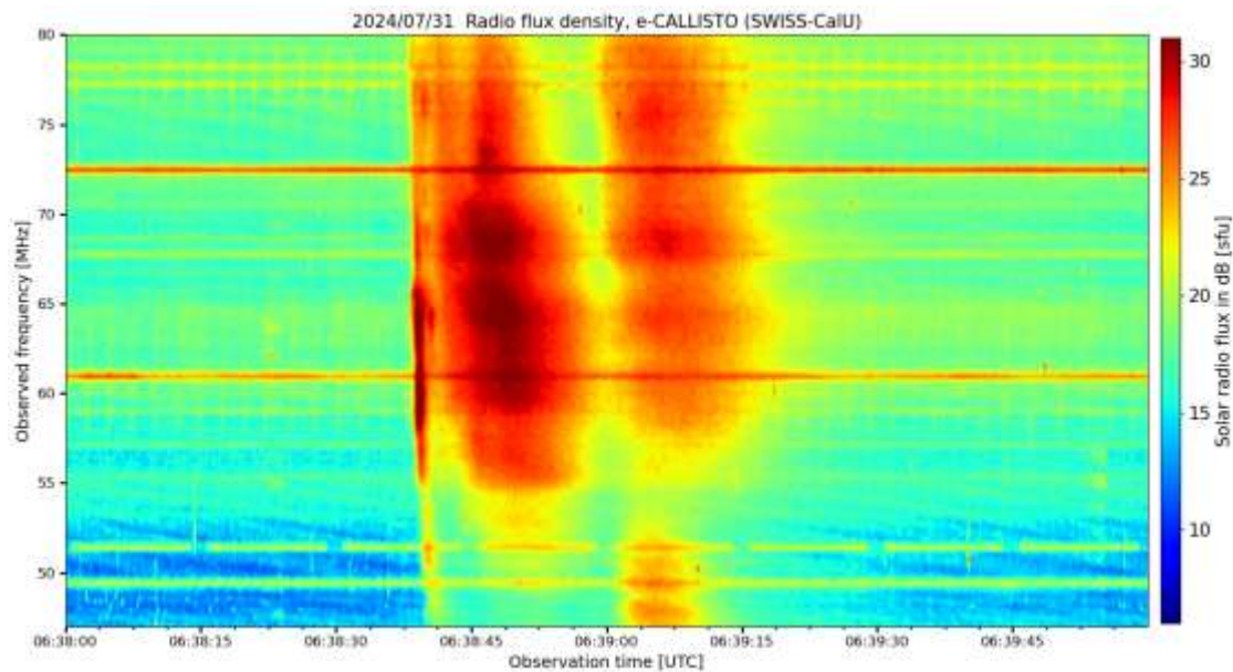
Fig. 15: Type III burst observed with CLP-5130-1N, data calibrated in SFU. Plot in Python3.
