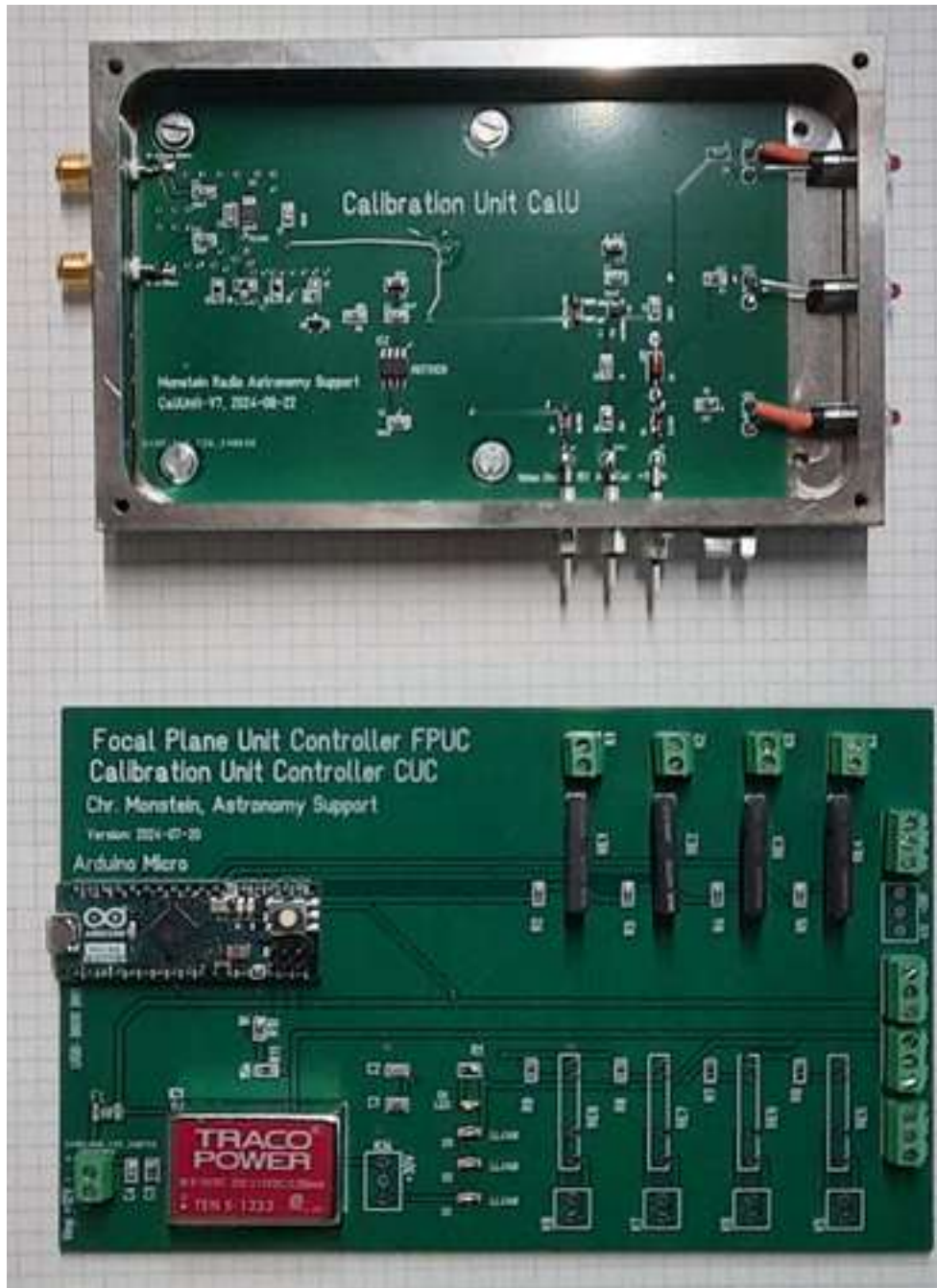
Fig. 7a: Image of outdoor calibration unit with open cover. Top left: antenna input, bottom left output input, bottom left output to LNA and finally to receiver. Right side three LED showing status of operation (antenna/calibration, noise excess and 15Vdc). Underneath feed through capacitor for antenna, noise and power.
