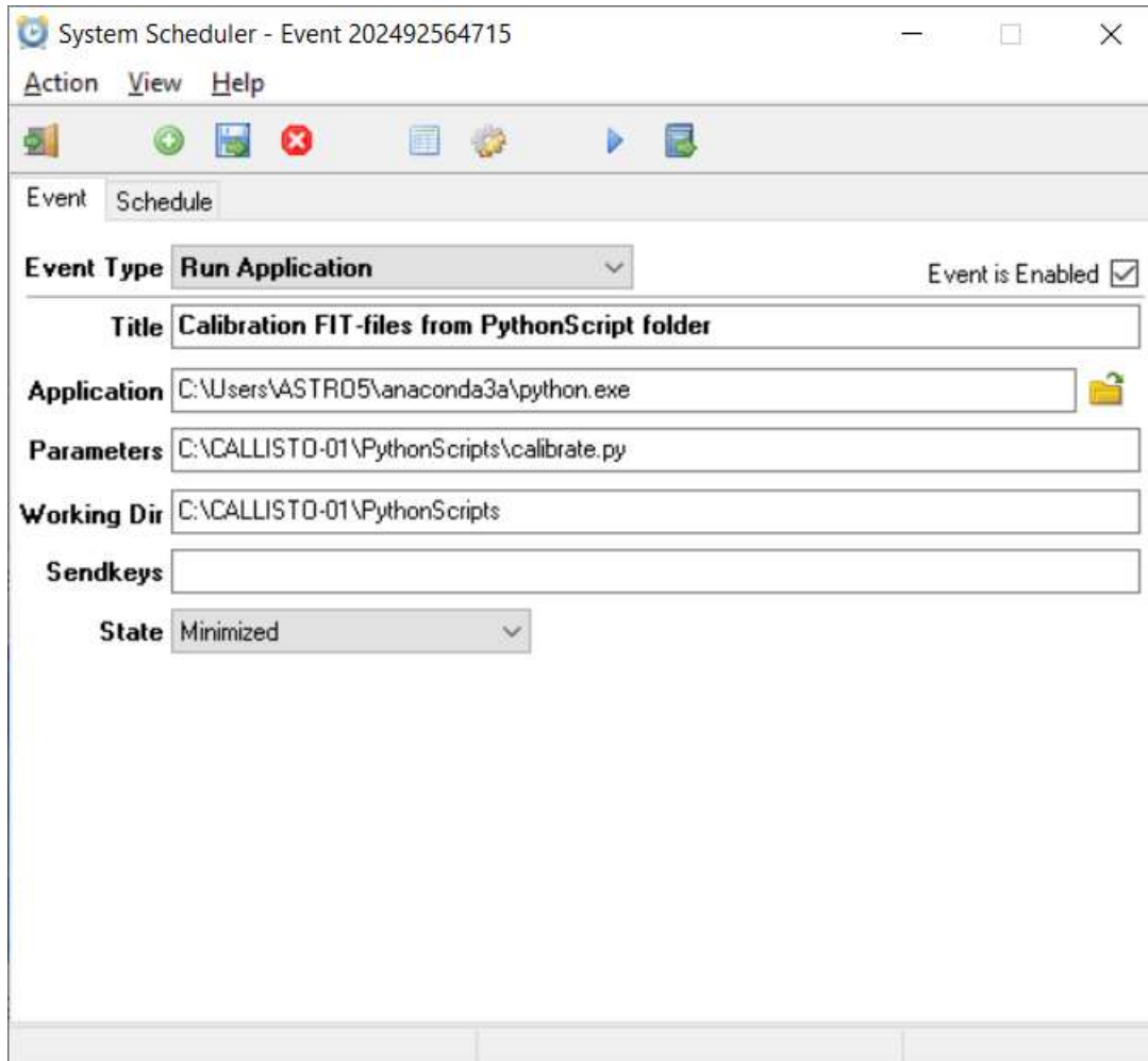
Fig. 18: Application configuration for FIT-file calibration. Path to Python.exe might be different for every user. You need to search for python.exe using file-explorer. Parameter-folder as well as working folder might also look different, depending on chosen drive and instrument-code = focus-code (00...63). From April 25 th , 2025 onwards replace python.exe by pythonw.exe and calibrate.py by calibrate.pyw!
