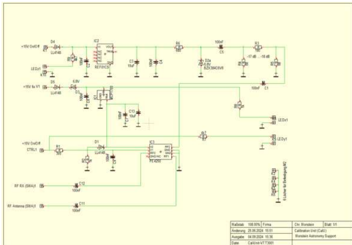
Fig. 2: Schematics calibration unit CalU with SPDT, Avalange noise diode and voltage regulators 10 V and 3.3 V.
